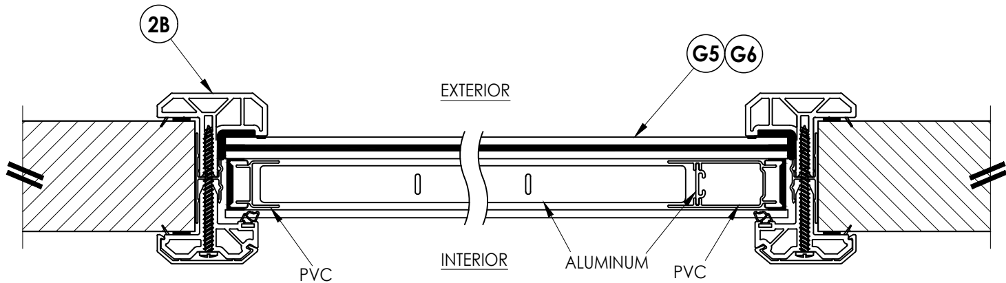
2 HORIZONTAL CROSS SECTION WARMEDGE OPERABLE BLIND NOTE: FIXED BLIND NOT SHOWN
